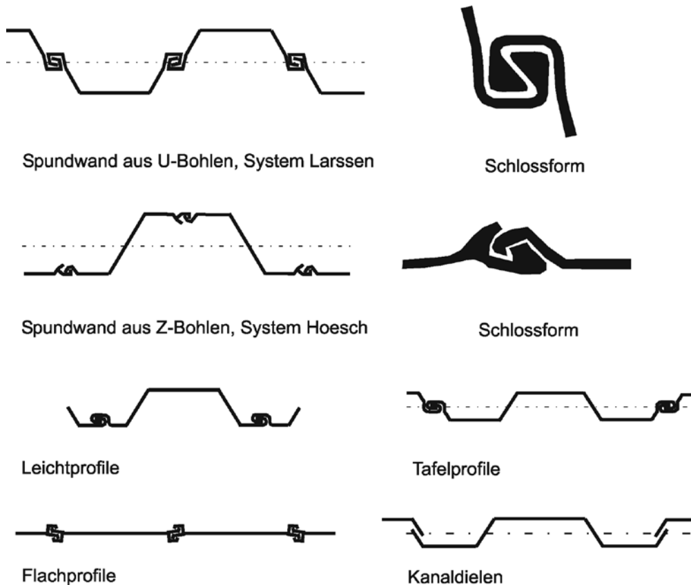
15-31 Spundwandprofile
