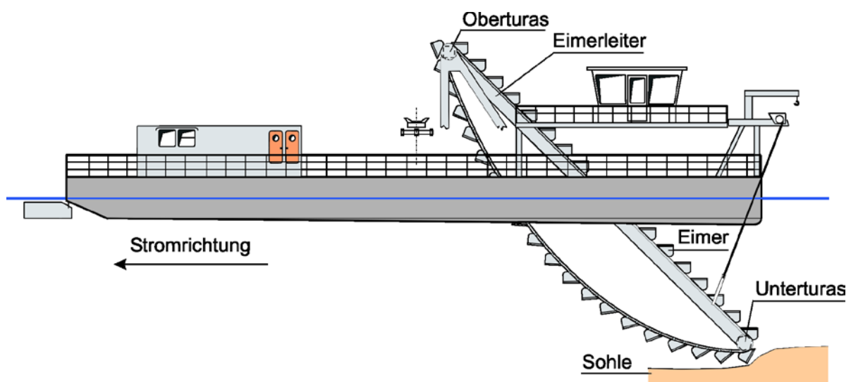
14-3 Eimerketten-Nassbagger
